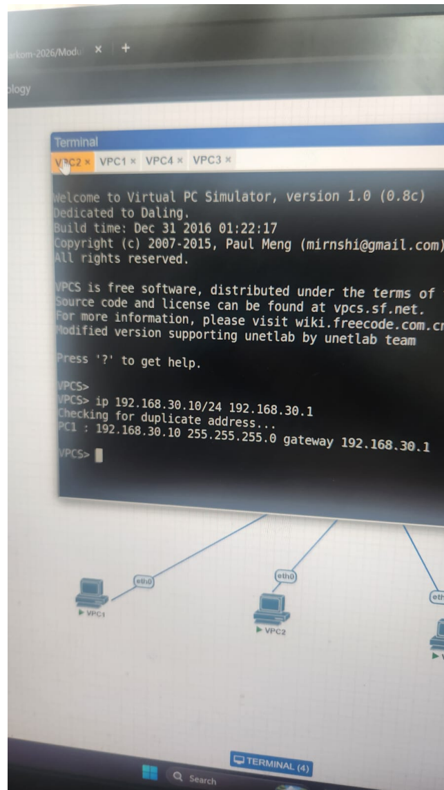
Gambar 8: IP manual Vlan 30
