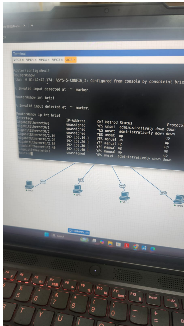
Gambar 3: interface brief Cisco router
